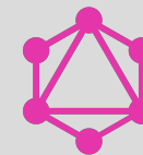
GraphQL
