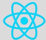
React native
